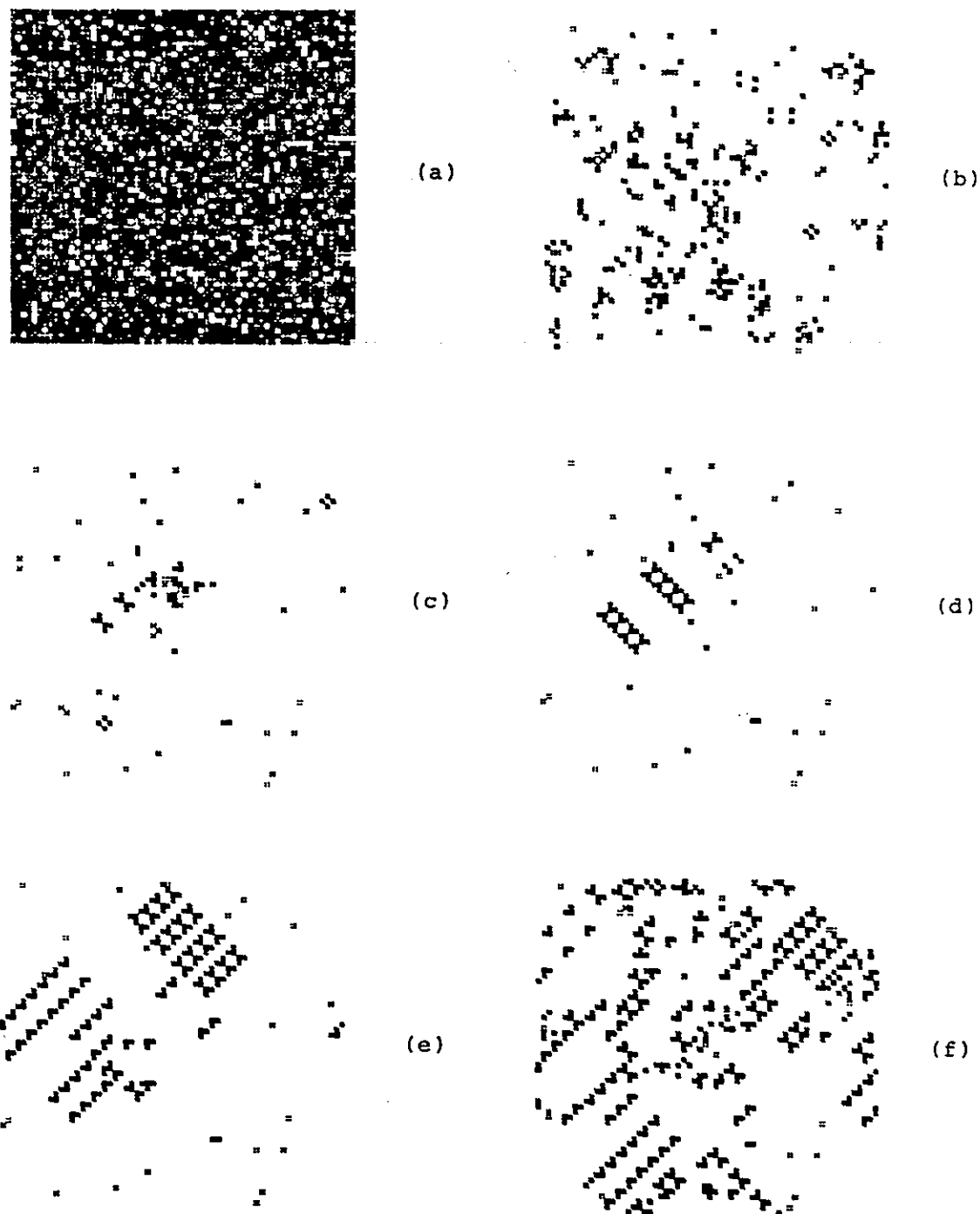
Figure 1: A cellular automaton with robust self-replicating patterns, discovered by Chris Langton. Figure (a) shows a random initial condition on a square lattice; the eight possible states are represented by distinct patterns of dots. As time evolves the density of blank states increases, as shown in (b) and (c). In (c) we already see the seeds of self-reproducing patterns; as time progresses these patterns grow by replicating themselves. There are several replicating patterns, which compete with each other for space, as shown in (d), (e), and (f).
